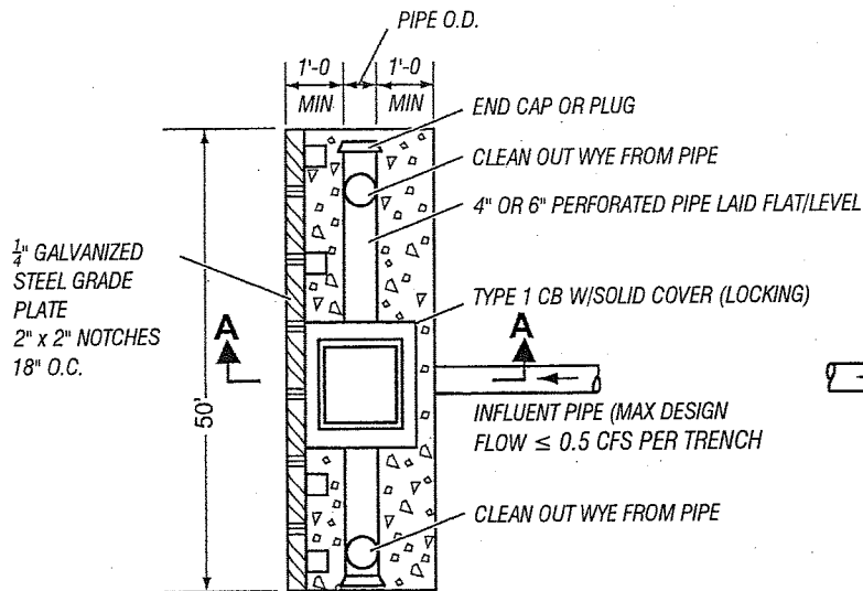
PLAN NTS
