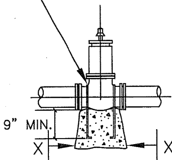
GATE VALVE
