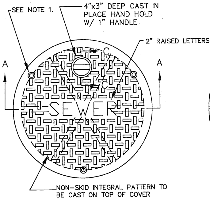
COVER PLAN
