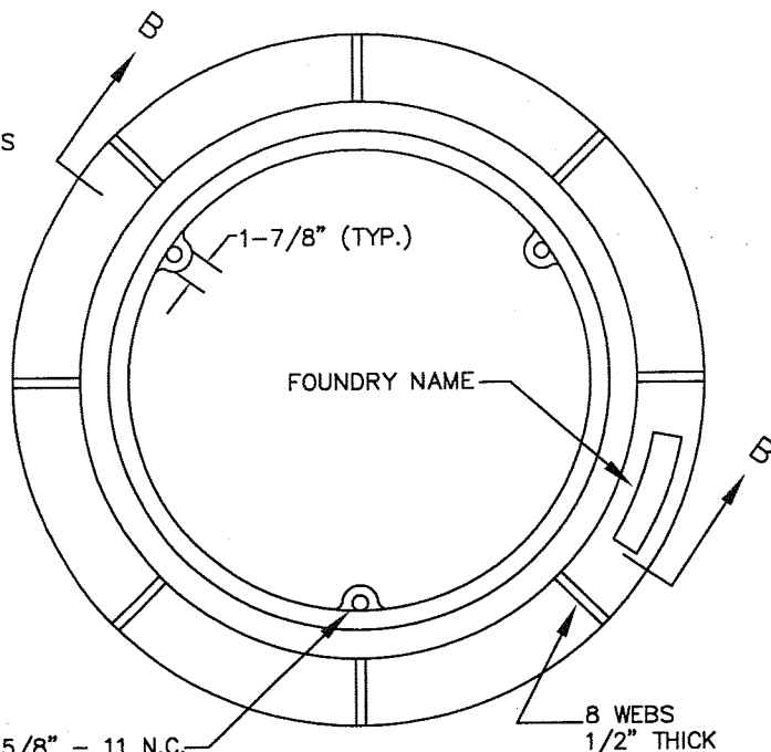
RING PLAN
