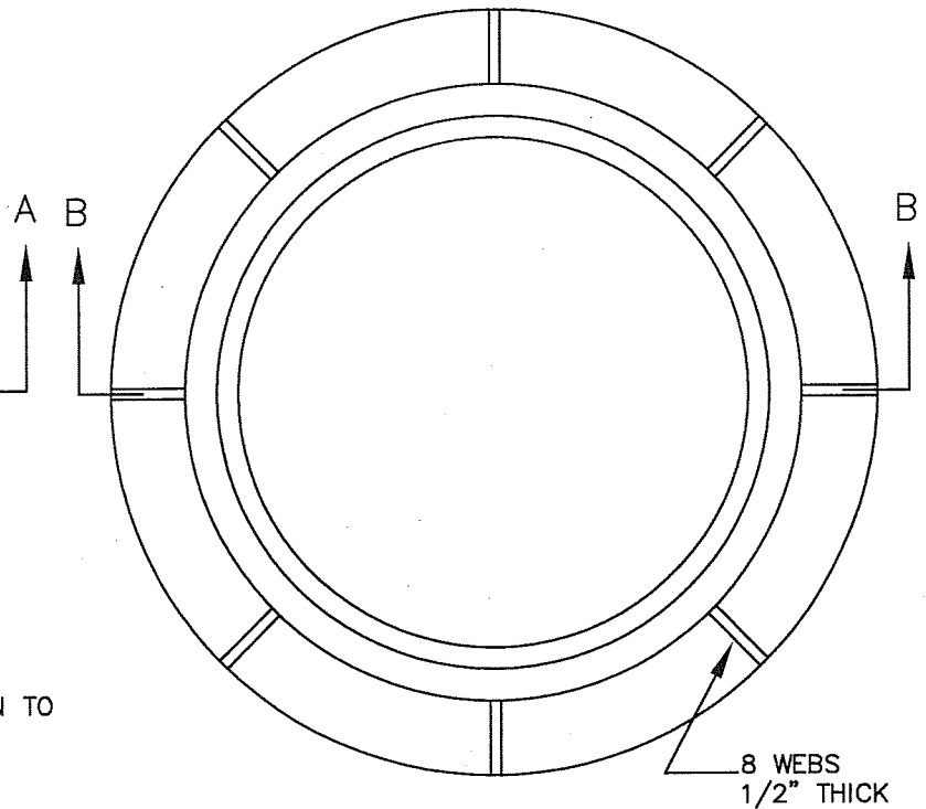
RING PLAN
